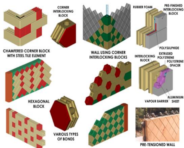
Figure 7- Hollow Core interlocking blocks
