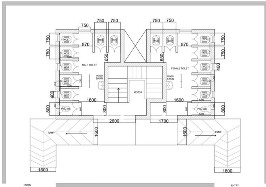
PLAN 1: Plan showing the existing toilets
