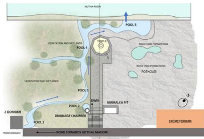
Figure 4. Plan of the study area (Source: Student report, drawn by Aayan Mulani)
