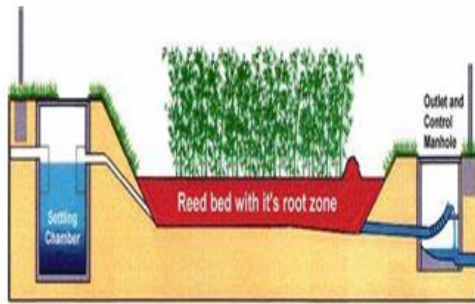
Figure 18. Root zone system
