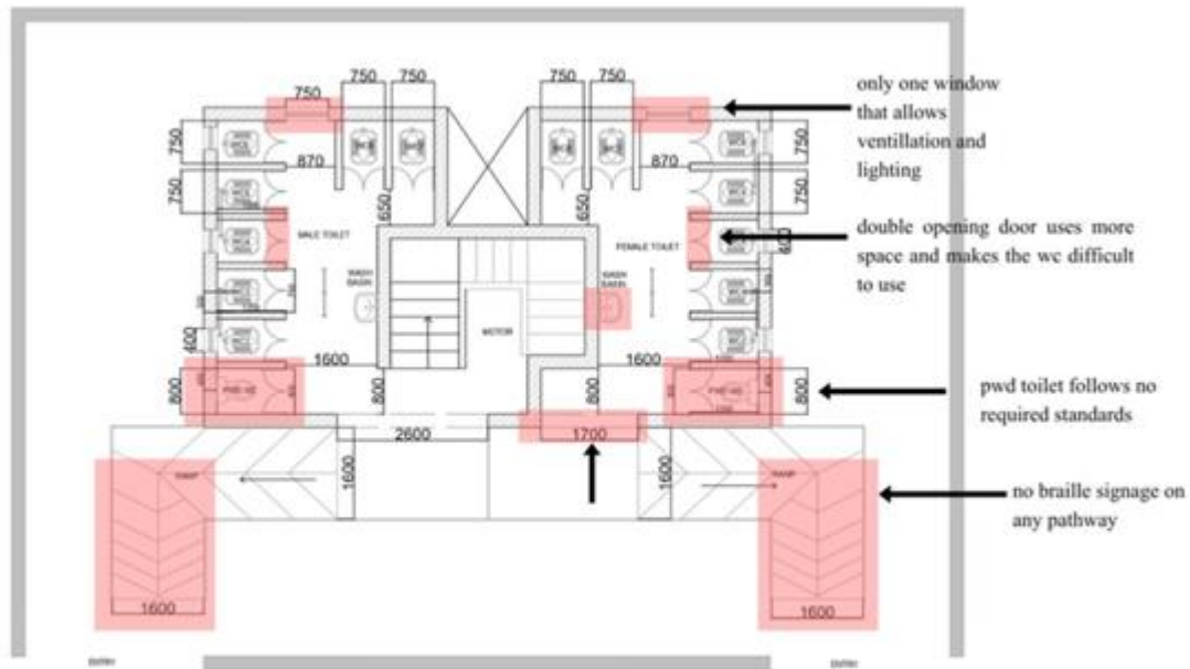
PLAN 2: Plan showing the problem areas of the existing toilets
