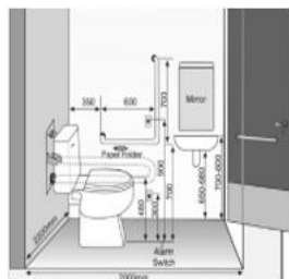
Figure 2. Dim in section
