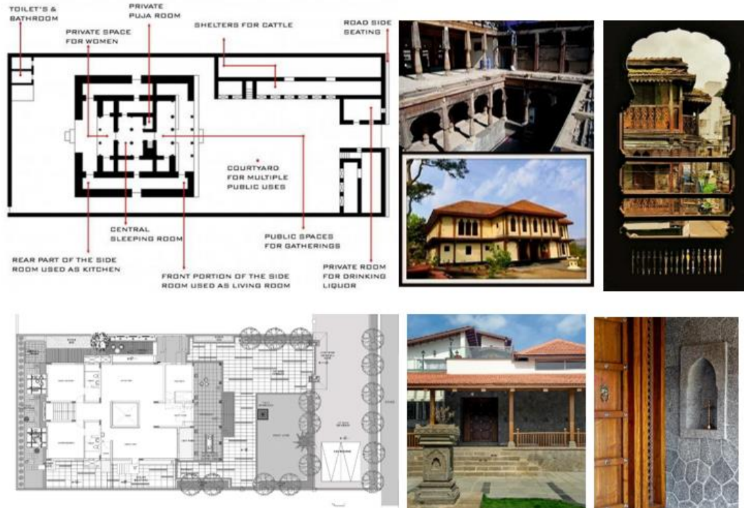
Figure 6. Typical plan of a Wada in Maharashtra (top left);
