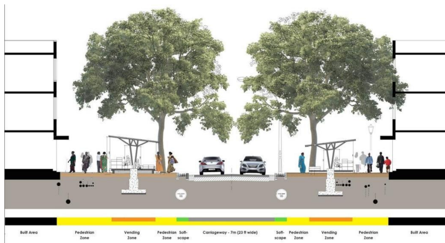
Figure 16: Proposed Section for the redevelopment of Gandhi Bazaar. Image Source: The Hindu
