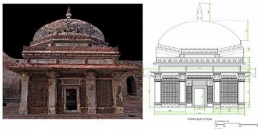
Figure 10: Laser scan derived blue print for Tomb of Imam Zamin, Qutub Complex.
