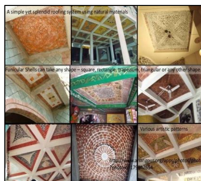
Figure 4. Refers to funicular shell roofs -construction techniques
